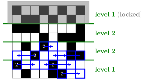
FIGURE 14. Optimizing the lower level 1 group.
