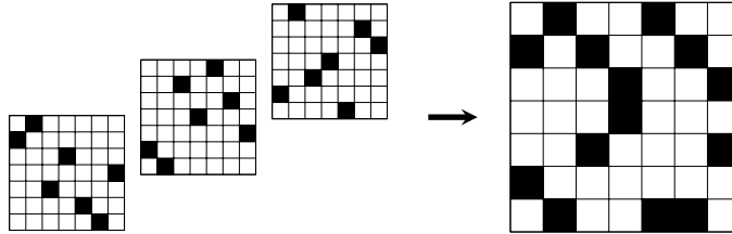
FIGURE 2. Exemplary aggregation of d permutations of [N] for the case d = 3, N = 7 .
