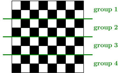
FIGURE 17. Groups with reordered columns.
