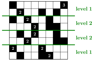
FIGURE 12. Levels of black blocks.
