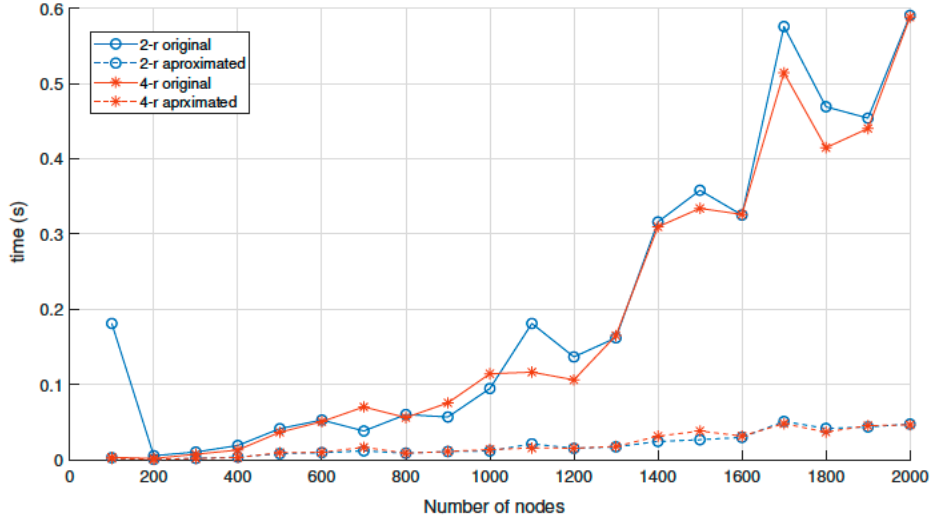
Figure 3. Eigenvalue calculation time
